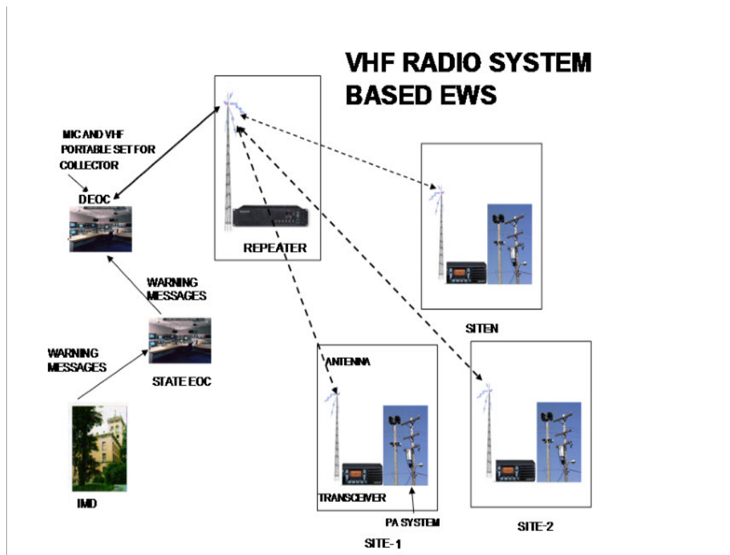
FIGURE 21: VHF BASED EARLY WARNING SYSTEM
