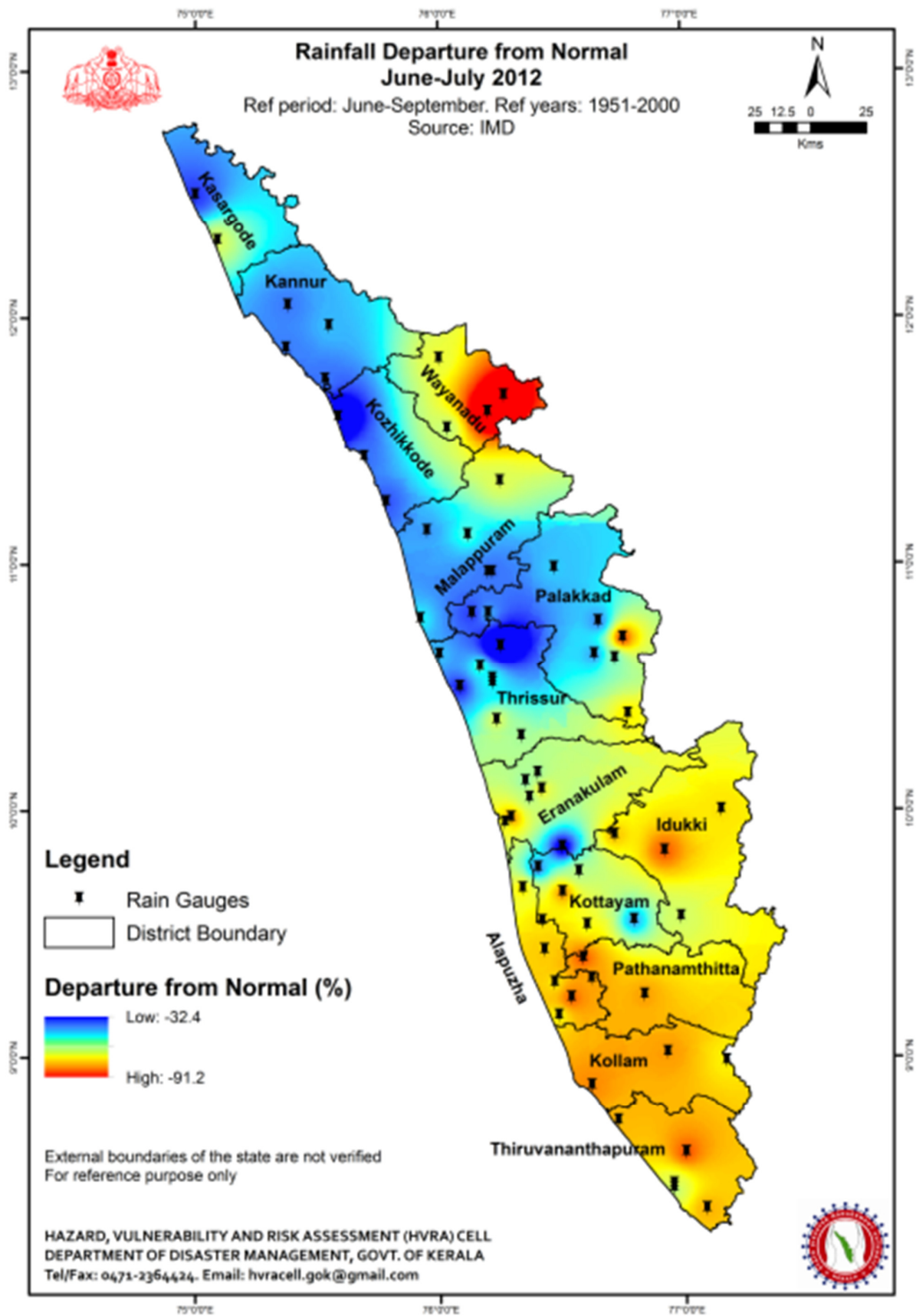
Figure 2: Map depicting the June-July 2012 rainfall departure from seasonal normal (June-September)
